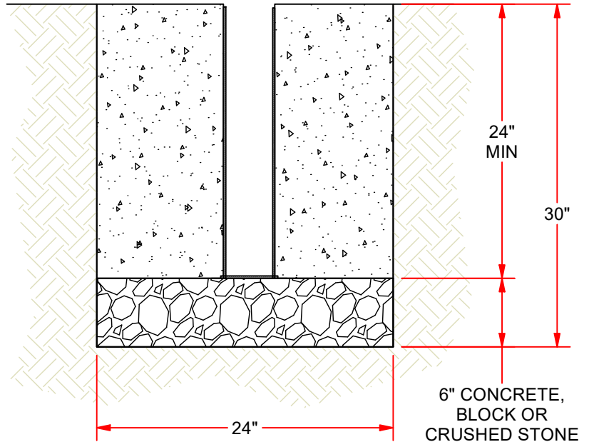
FOOTING DETAIL
